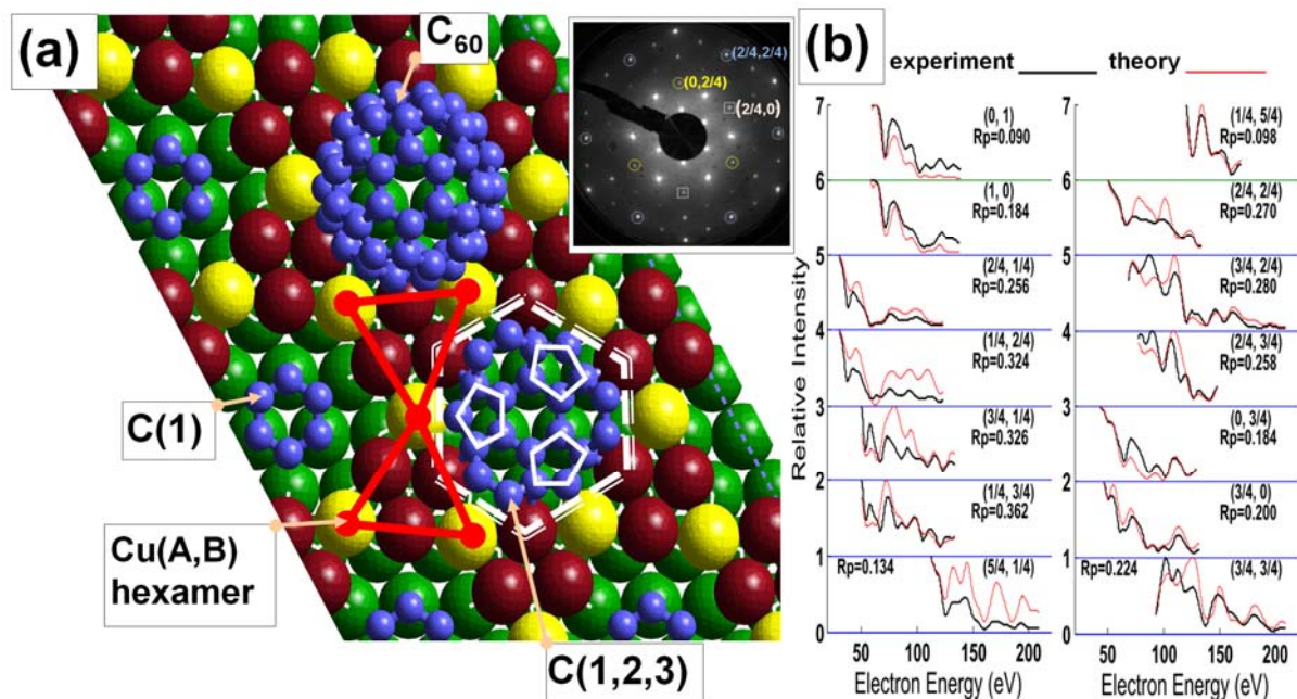
Figure 3 (a) The reconstructed model of the C_{60}/Cu(111) interface. Color scheme: 1st-layer Cu(A)(red) and Cu(B)(yellow), 2nd-layer Cu(green), C atoms(blue). C(N) , N=1,2,\dots , denotes the bottom N-th C layer of a C_{60} . The C(1) layer, C(1,2,3) portion, and a full C_{60} are all depicted. The top Cu layer is significantly distorted, leading to alternating rotation of Cu(A,B) hexamers (red solid line) on a honeycomb sublattice and a distorted Cu(A) hexagon(white dashed line). (b) Selected LEED I-V beams and their tensor LEED fitting. The inset shows a typical LEED pattern, with some beam indices labeled.
