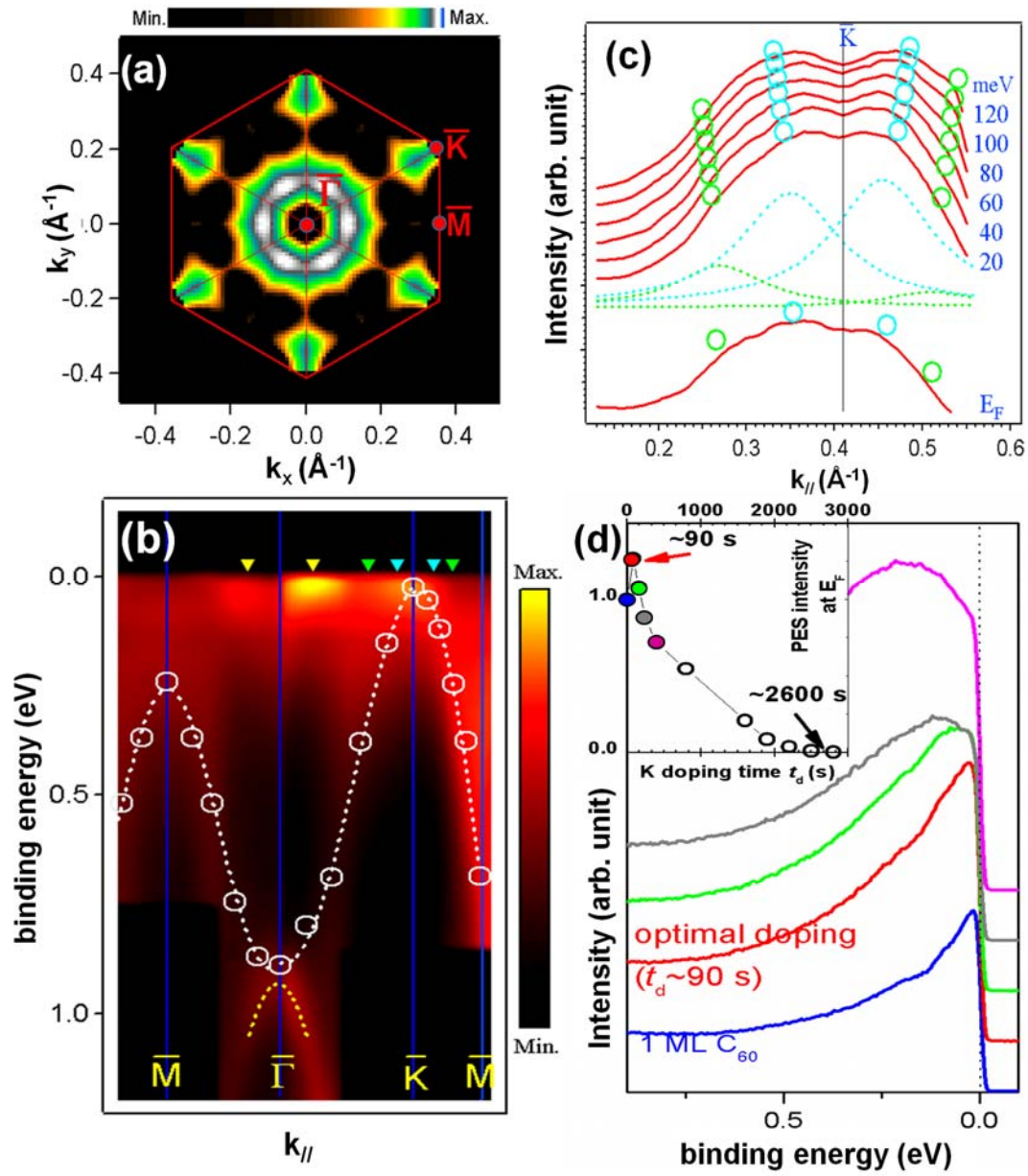
Figure 1 (a) Fermi surface (FS) mapping of 1 ML C 60 . At least two regions of FS crossings were observed around \bar{\Gamma} and \bar{K} . (b) Band dispersion along \bar{\Gamma} - \bar{M} and \bar{\Gamma} - \bar{K} . FS crossings are marked by three pairs of colored triangles. The white circles denote the calculated LUMO-derived bands and the white dashed line is a guide to the
