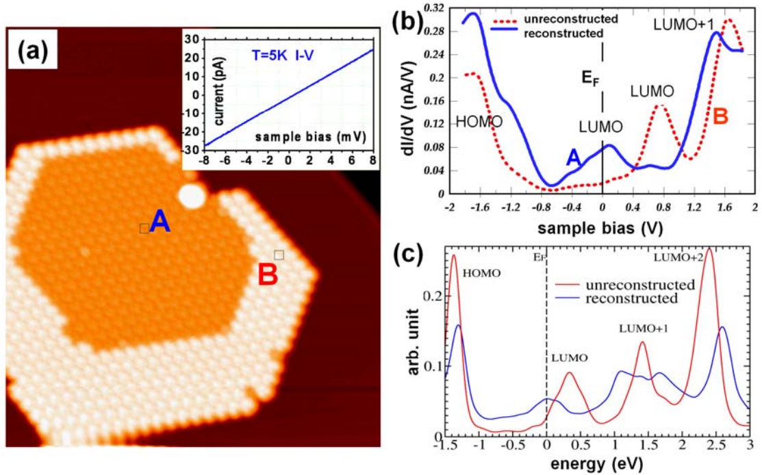
Figure 2 (a) A "core-shell" island (35 nm × 35 nm). (b) STS spectra show a dramatic shift of the LUMO band in the reconstructed core vs. unreconstructed shell region. T= 77 K. (c) Calculated C 60 PDOS of the unreconstructed and reconstructed (r-fcc) C 60 /Cu(111) with 0.1 eV Gaussian broadening. The inset of 2(a) shows no energy gap near E F in STS at ~5 K.
